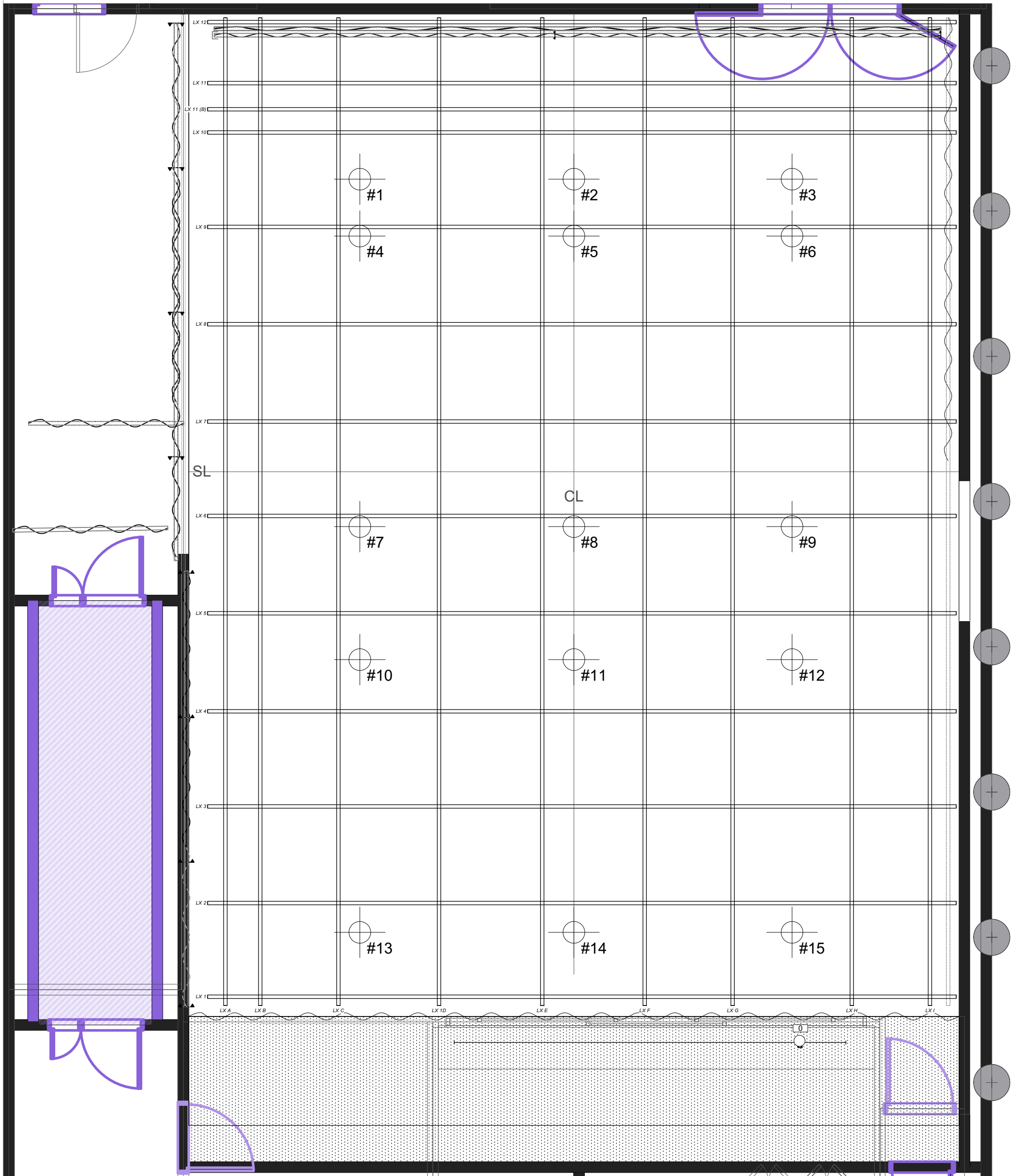
1 NBT_GridPlan_RiggingPoints Scale: 1:50
